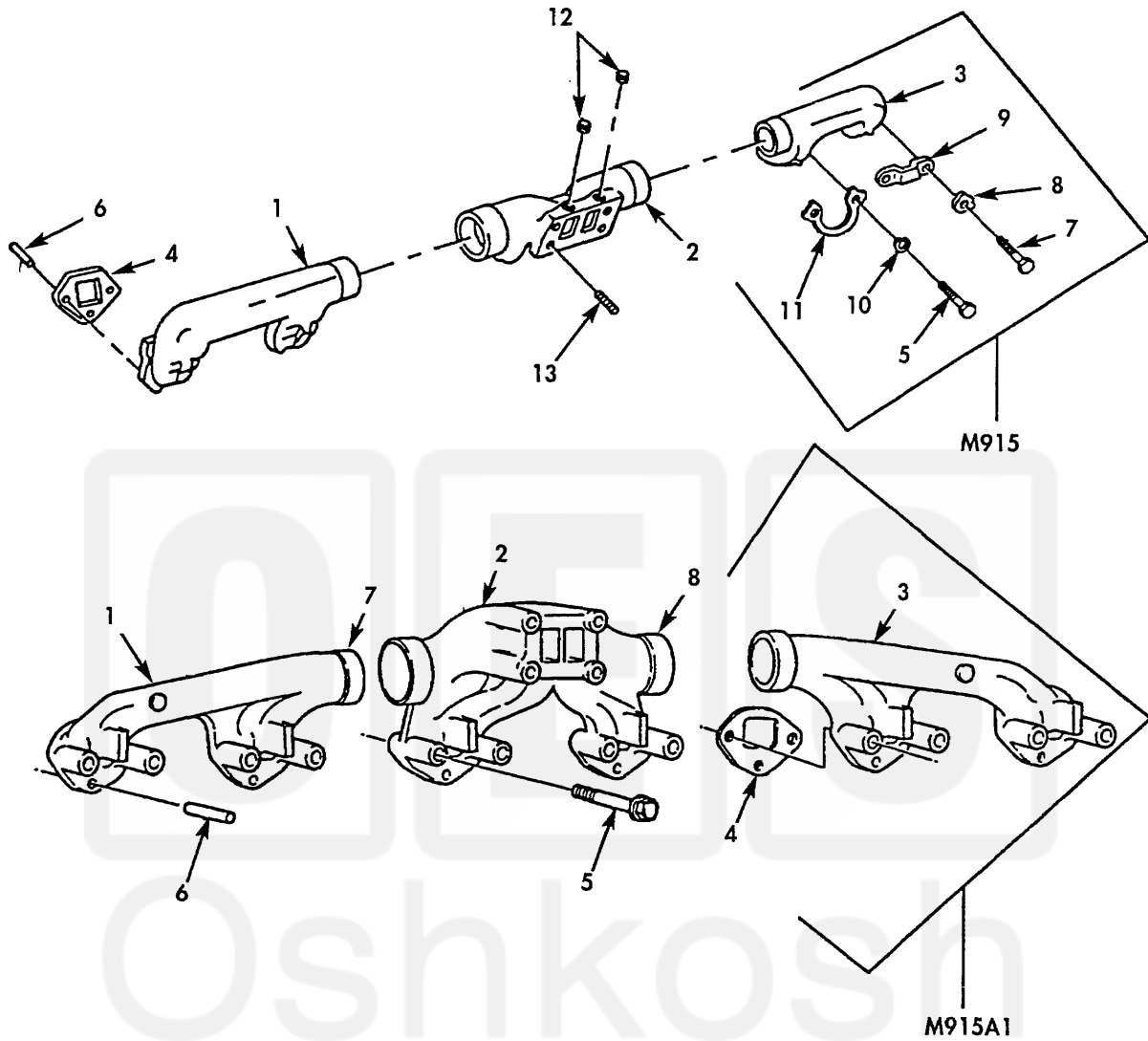
Figure 15. Exhaust Manifold.
